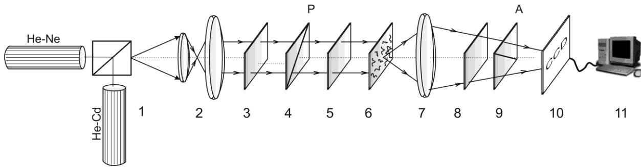
Fig. 1. Optical scheme of "two-wave" spectral-selective stockpolarimeter
